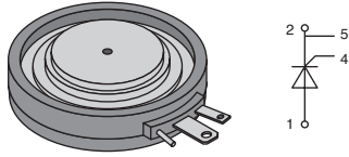
Thyristor
